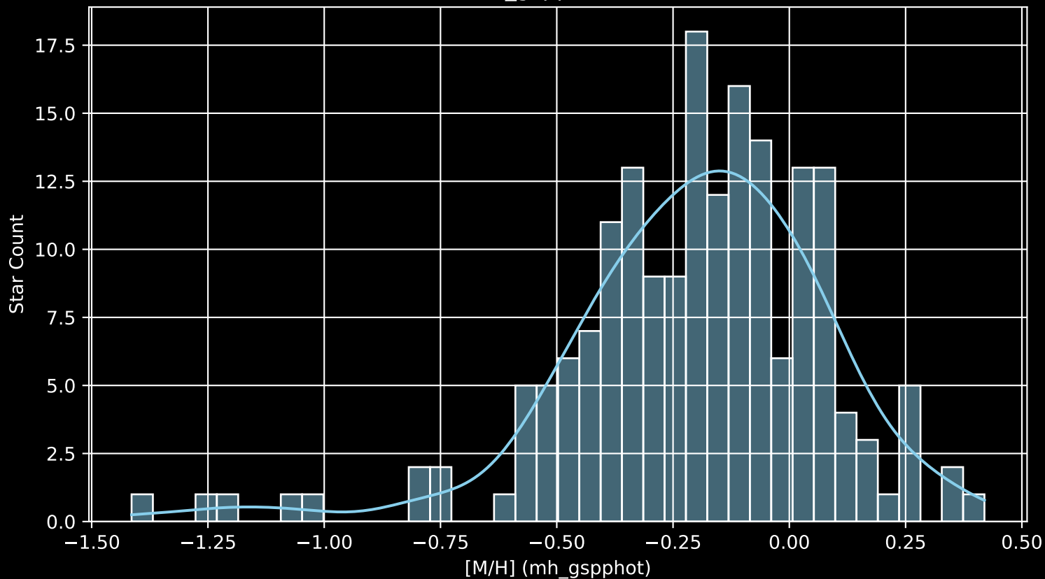
APOGEE DR17 Field: [194+24_MGA [M/H] (mh_gspphot) (n= 183)
