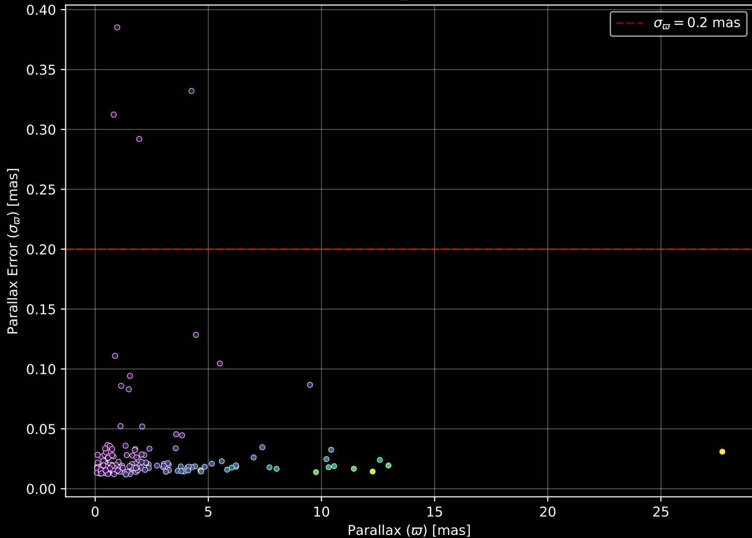
APOGEE DR17 Field: [194+24_MGA] Parallax Quality (n= 185)
