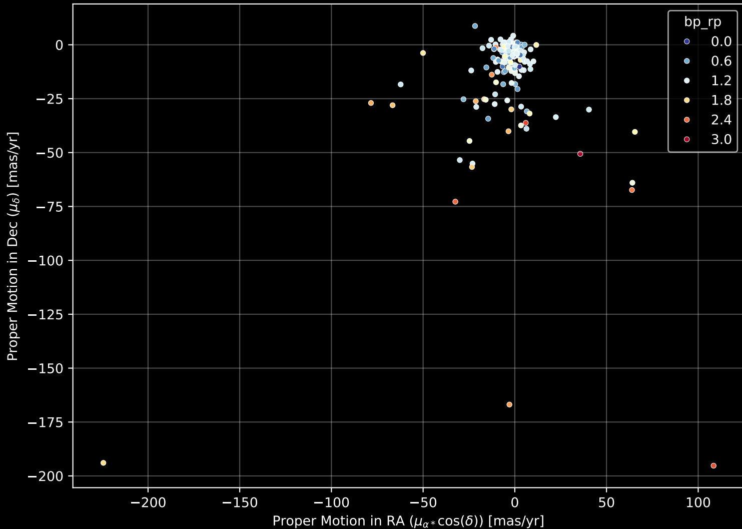
APOGEE DR17 Field: [194+24_MGA] Proper Motion Diagram (n= 185)
