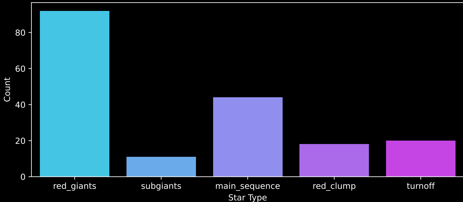
APOGEE DR17 Field: [194+24_MGA] Count plot of Star Type
