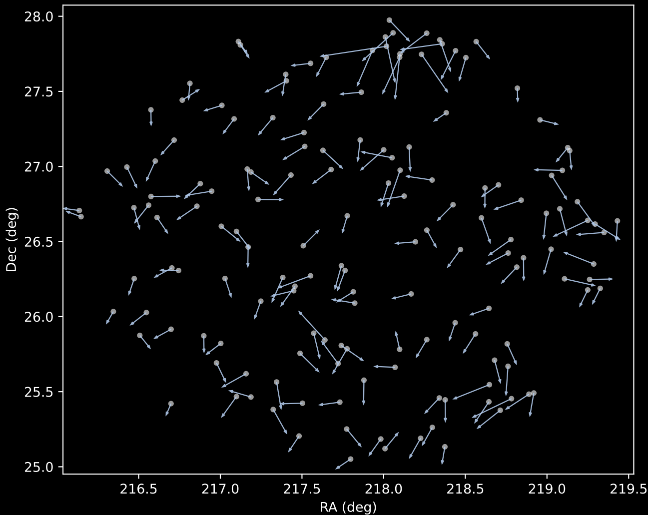
APOGEE DR17 Cluster 1 Proper Motion Vectors (n=155)
