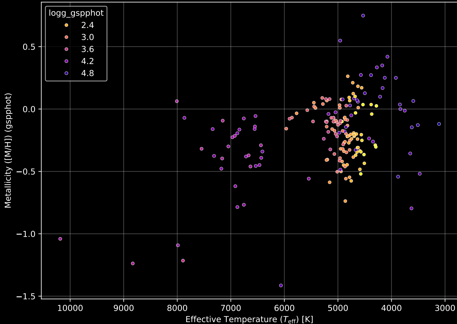
APOGEE DR17 Field: [194+24_MGA] Stellar Population Parameters (n= 185)
