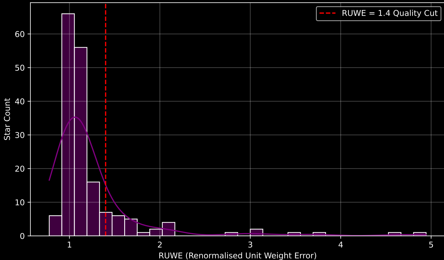
GAPOGEE DR17 Field [194+24_MGA] RUWE Distribution (n= 176)
